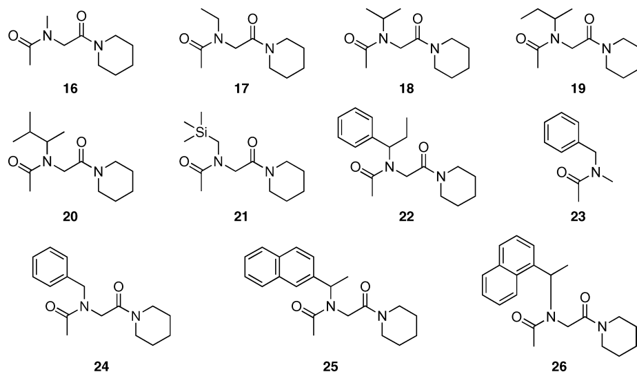
Figure 6. Structures of the peptoid model systems ( 16–26 ) designed to probe steric interactions.
