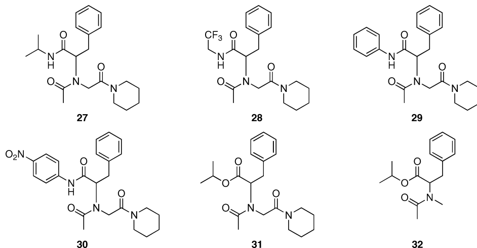
Figure 7. Structures of the peptoid model systems (27–32) designed to probe hydrogen bonding interactions.
